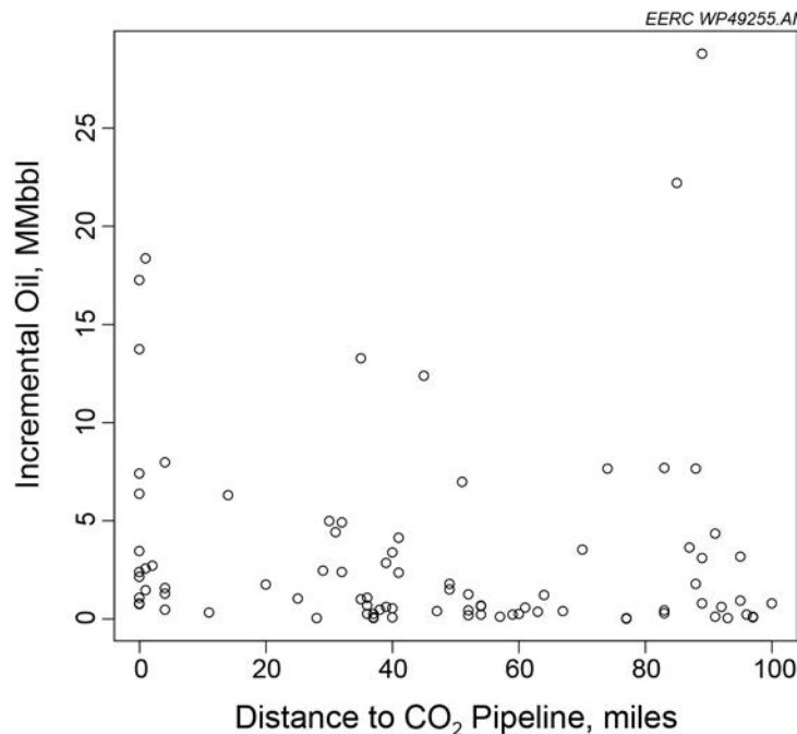
Figure 13. Relationship between incremental oil (RF = 0.08) and distance from units to nearest CO 2 pipeline.
