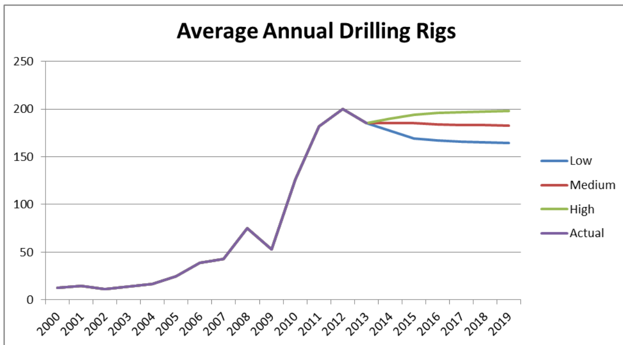
Figure 2: Average Annual Rig Counts, North Dakota, 2000 through 2019
