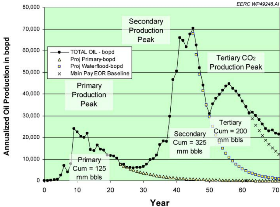
Figure 1. Example of field decline curve (from Hill and others, 2013).
