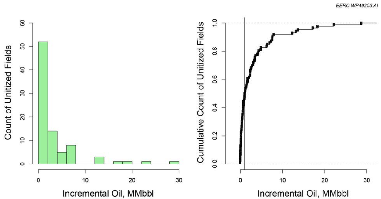
Figure 10. Distribution of estimated incremental oil as a) histogram and b) cumulative distribution plot.
