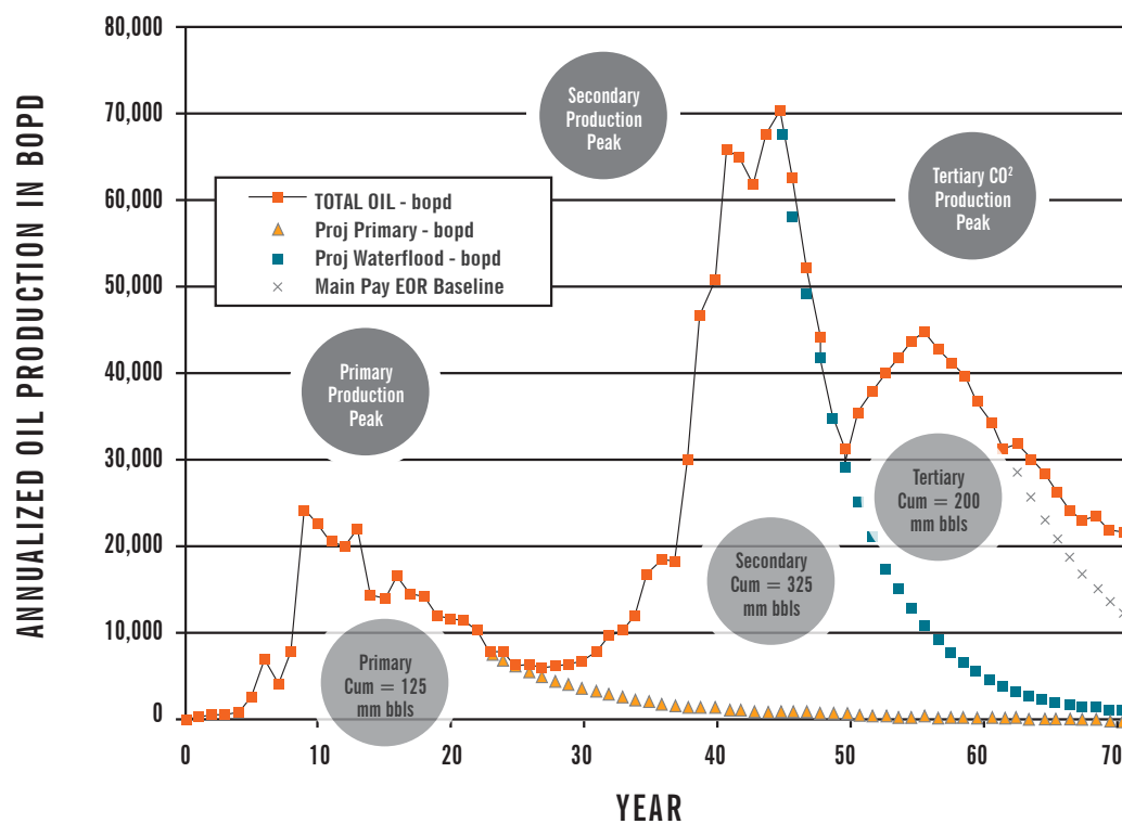
Figure 35: Example of field decline curve Source: EERC
