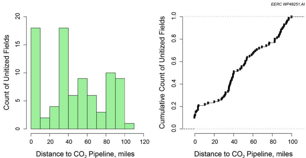
Figure 8. Distribution of distances to CO 2 pipelines as a) histogram and b) cumulative distribution plot.
